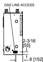
SL-750TR & TRS Side View
